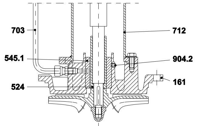
Lubrificazione bronzina e tenuta meccanica dall'esterno Bushing and mechanical seal lubrication by means of external fluid supply "D" exec.
