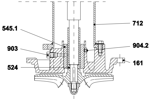
Lubrificazione bronzina dall'esterno Bushing lubrication by means of external fluid supply "C" exec.
