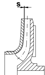
Fig.7 RG pump section
