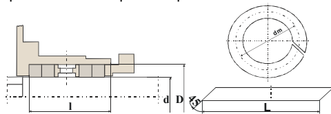
Fig.5 Tenue garniture
