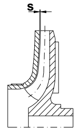
Fig.7 Section pompe RG
