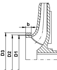
Fig.6: RD pump section
