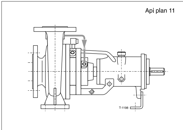
FLUSSAGGIO DALLA MANDATA Recirculation from pump case to seal
