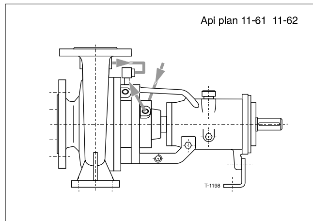
FLUSSAGGIO DALLA MANDATA E QUENCH POSTERIORE Recirculation from pump case to seal and quench
