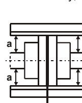
Fig. 2 Coupling alignment
